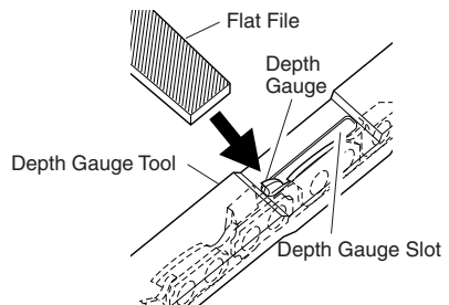
Figure 22 - Depth Gauge Tool On Chain
