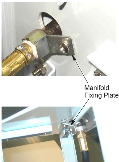
Figure 7 - Attaching Manifold Fixing Plate to Post Support
