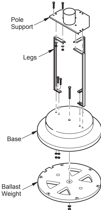
Figure 1 - Base Assembly
