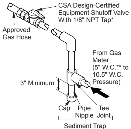
Figure 4 - Gas Connection
