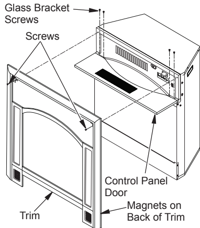
Figure 8 - Removing Trim
