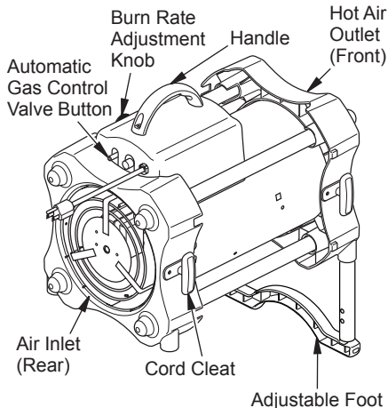
Figure 1 - 55/85/125,000 Btu/Hr Models
